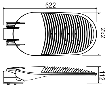
KTSL5801A(M) 50-100W
