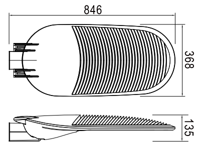
KTSL5801A(L) 100-170W
