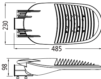
KTSL5801A(S) 20-50W
